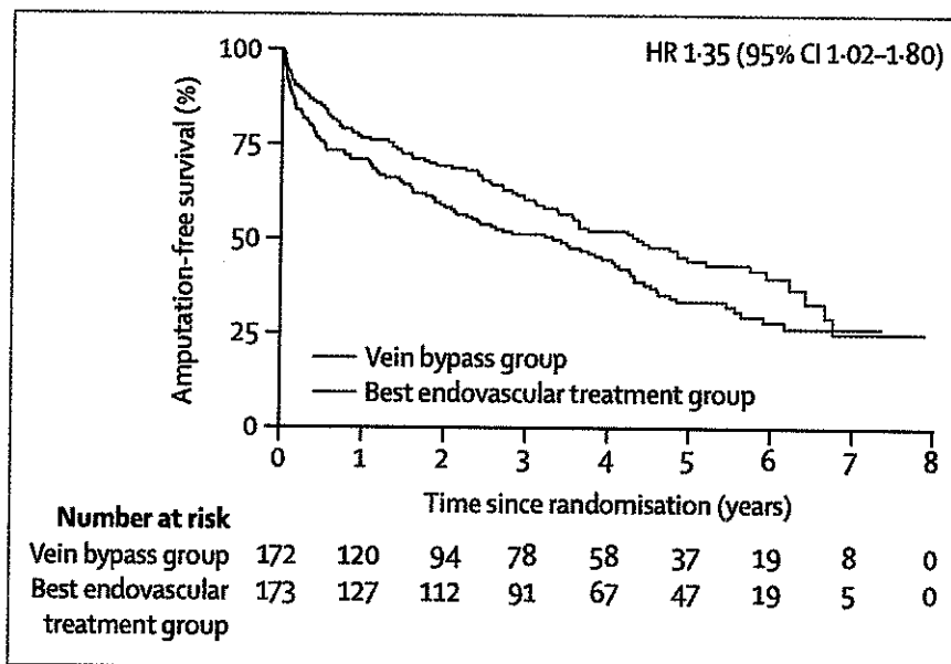
Figure 2: Amputation-free survival Kaplan-Meier curve
