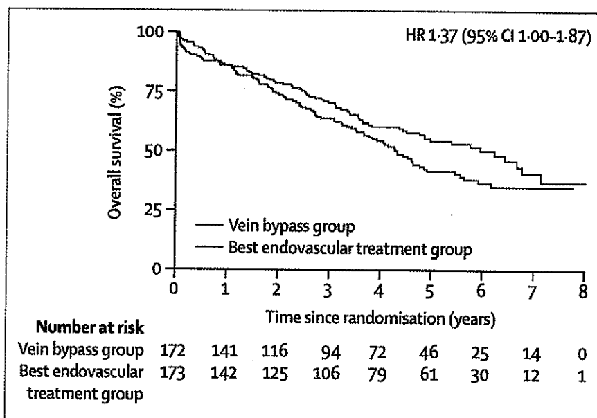
Figure 3: Overall survival Kaplan-Meier curve
